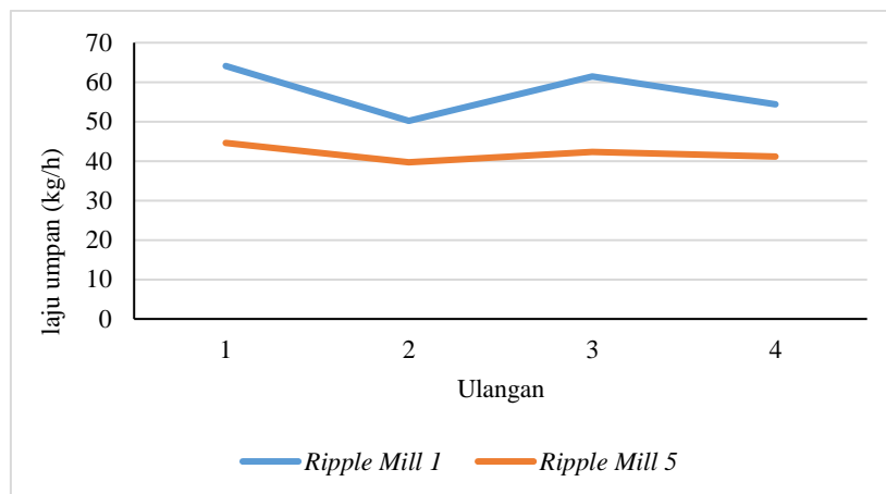
Gambar 1 Laju umpan Ripple Mill
