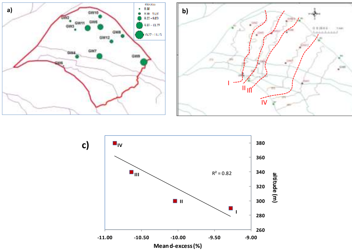
Figure 1. (a) The d-excess distribution in the study area, (b) Recharge water line from I to IV and the groundwater well locations, (c) mean d-excess as a function of recharge line altitude.
